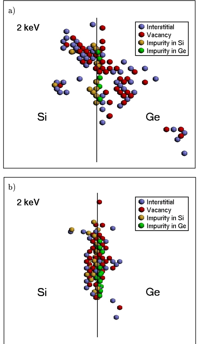
FIG. 1. Final distribution of damage in two different 2 keV cascades started in the (100) interface plane of a Si/Ge interface. Note that in both events there are more impurities on the Si than Ge side of the interface after the cascade.
