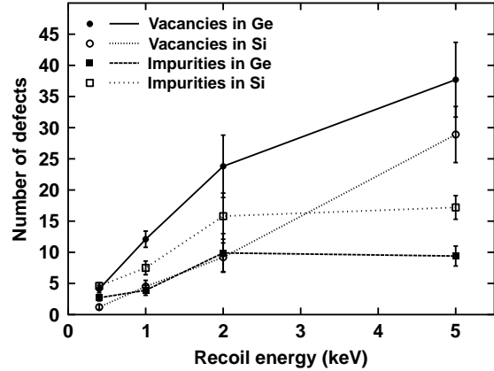
FIG. 2. Energy dependence of the production of defects in cascades initiated close to the (100) interface plane in Si/Ge systems.
